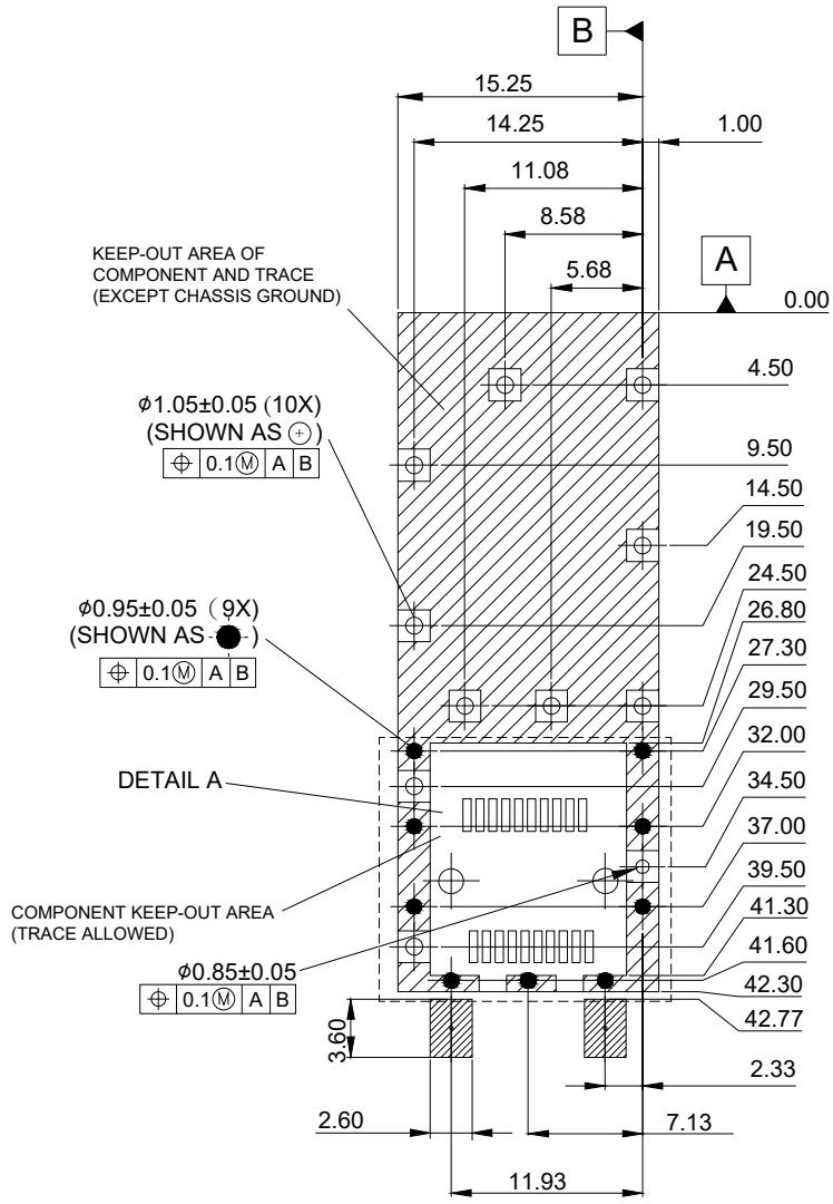
RECOMMENDED PCB LAYOUT (PCB Thickness 1.60mm)
